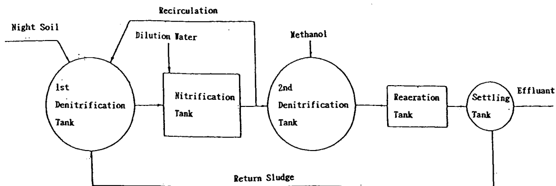
Figure 2. Biological denitrification process for nightsoil
