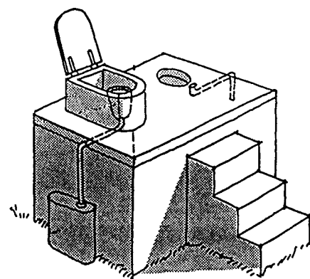
Figure 2. LASF toilet
